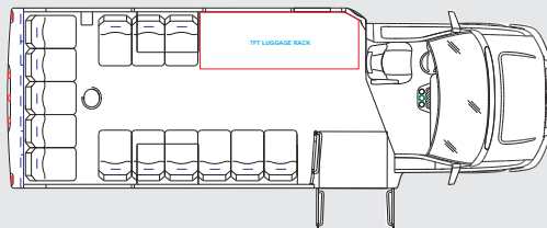
24ft, 165" WB - 19 Passenger
