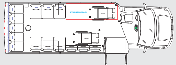
27ft, 191" WB - 23 Passenger
