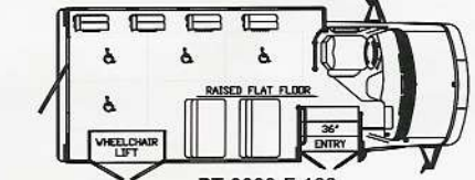
PT 2000-F-103 12 PASSENGER & 1 W/C OR 4 PASSENGER & 4 W/C
