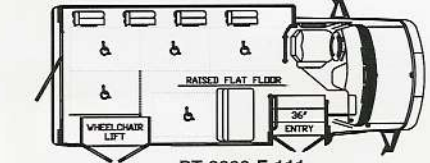
PT 2000-F-111 10 PASSENGER & 2 W/C OR 2 PASSENGER & 5 W/C
