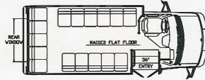
VIP 2000-D-100 16 PASSENGER
