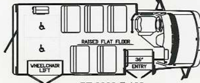
PT 2000-F-102 12 PASSENGER & 1 W/C OR 10 PASSENGER & 2 W/C
