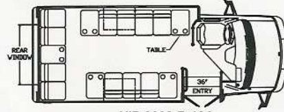
VIP 2000-D-104 11 PASSENGER
