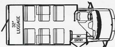
VIP 2000-B-103 12 PASSENGER
