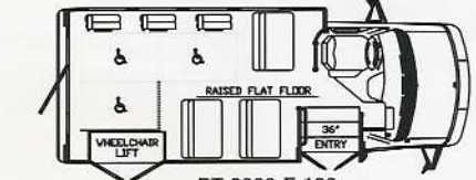
PT 2000-F-100 12 PASSENGER & 1 W/C OR 6 PASSENGER & 3 W/C
