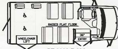
PT 2000-F-104 12 PASSENGER & 1 W/C OR 8 PASSENGER & 2 W/C
