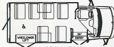
PT 2000-F-119 12 PASSENGER & 1 W/C
