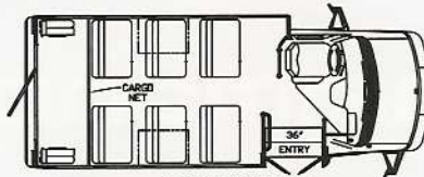
VIP 2000-C-109 12 PASSENGER & LUGGAGE OR 16 PASSENGER
