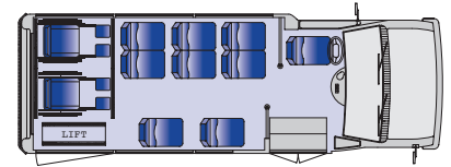
8 passengers plus 2 wheelchairs and driver. DRW
