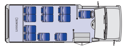
10 passengers plus driver, with rear luggage area. DRW
