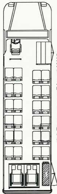
26 Passenger Plus 2 W/C
